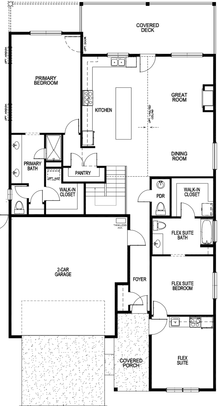
MAIN LEVEL
